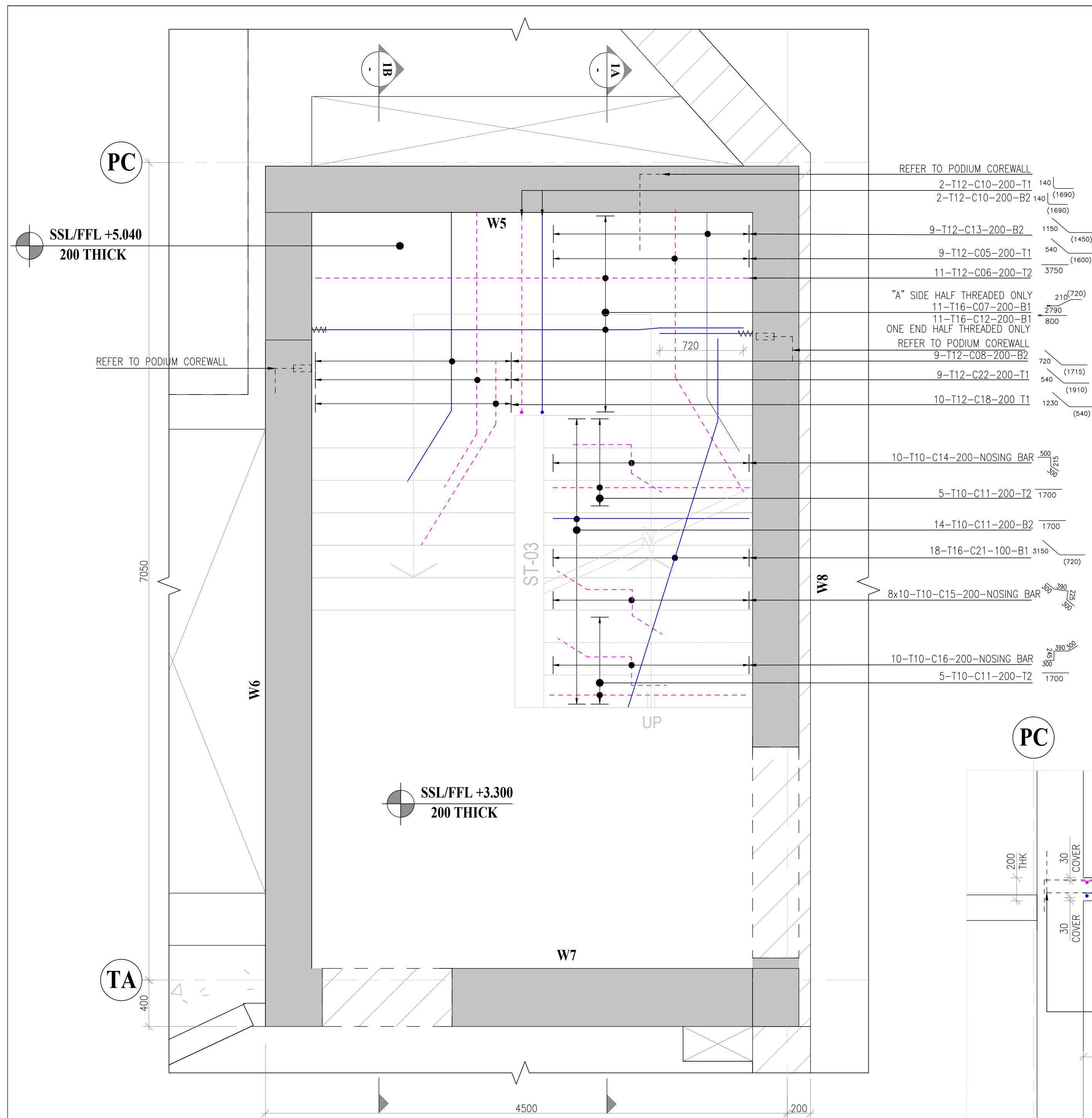
PLOT-4 STAIR CASE 03 REINFORCEMENT DETAILS FROM +3.300 TO +5.040 LEVEL GRIDS BET. (TA-PC)-(P12) SCALE: 1:25
